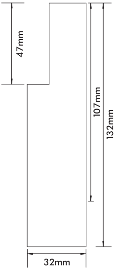
Solid Door Frame White Primed 107mm or 132mm
