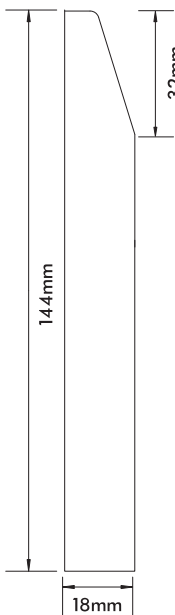
Chamfered Skirting 144mm x 18mm x 4200mm
