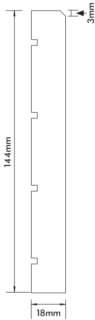
Contemporary Skirting 144mm x 18mm x 3600mm
