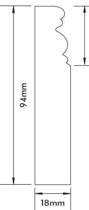
Moulded Architrave 94mm x 18mm
