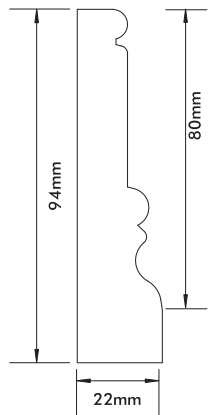
Grange Architrave 94mm x 22mm
