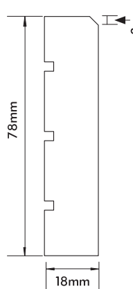
Contemporary Architrave 78mm x 18mm
