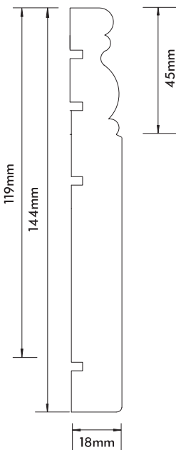
Moulded Skirting 119/144mm x 18mm x 3600mm
