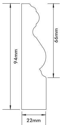
Victorian Architrave 94mm x 22mm
