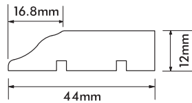
Door Stop 12 x 44mm (included in door frame set)
