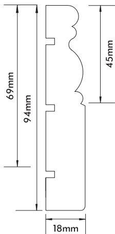
Moulded Architrave 69 / 94mm x 18mm
