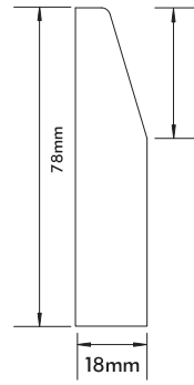
Chamfered Architrave 78mm x 18mm
