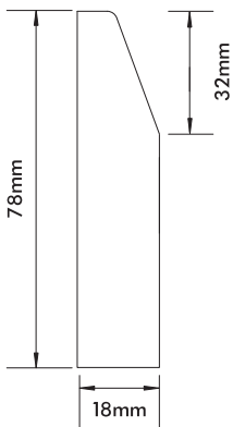
Chamfered Architrave 78mm x 18mm
