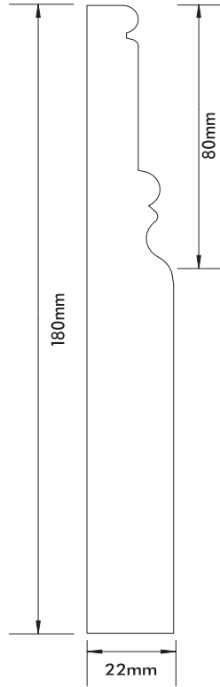
Grange Skirting 180mm x 22mm x 4200mm
