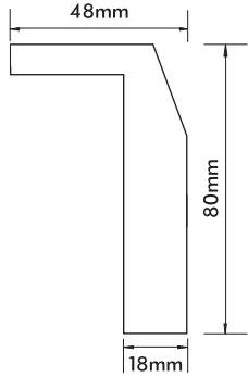
Adjustable Chamfered Architrave 80mm x 18mm
