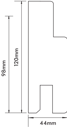
Adjustable Door Frame 98mm/120mm x 44mm
