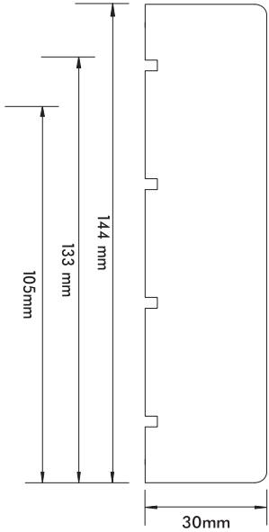
Door Frame 105mm/133mm/144mm x 30mm
