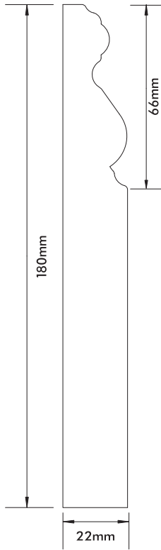
Victorian Skirting 180mm x 22mm x 4200mm
