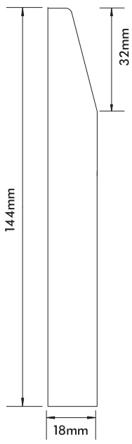
Chamfered Skirting 144mm x 18mm x 3600mm
