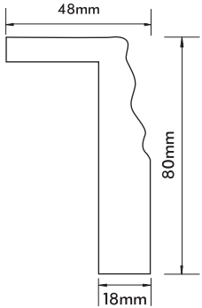
Adjustable Moulded Architrave 80mm x 18mm
