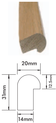
Oak Hockey Stick 20mm x 31mm
