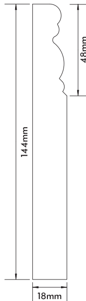
Moulded Skirting 144mm x 18mm x 4200mm
