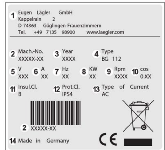
Fig. 6 Data on motor type plate.
